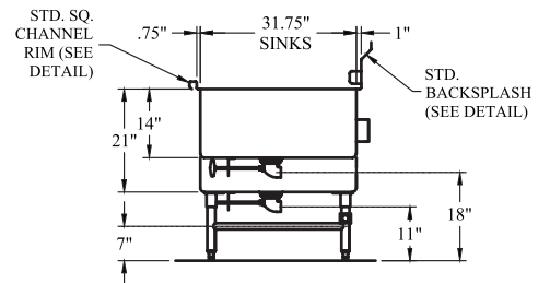
SECTION "A"
