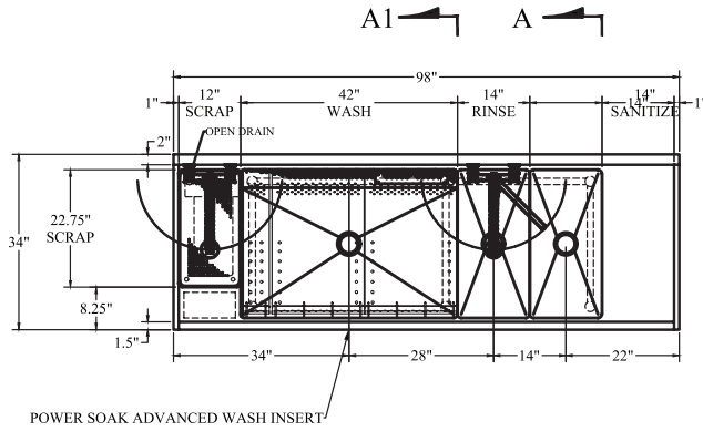
POWER SOAK ADVANCED WASH INSERT
