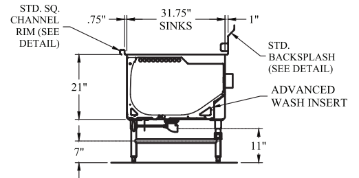
SECTION "A1"
