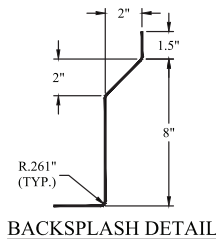
BACKSPASH DETAIL
