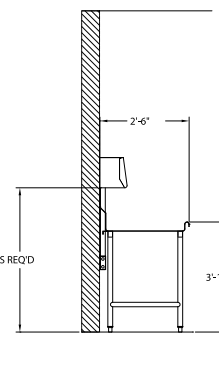
TYPICAL SECTION VIEW
