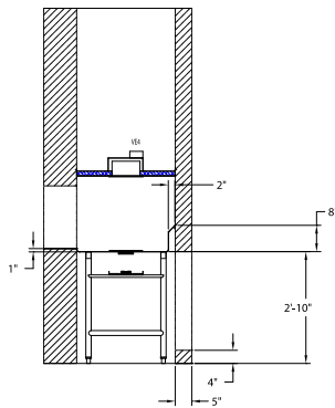
TYPICAL SECTION VIEW
