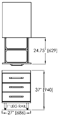
Model C11043-27TE Increases standard 24" refrigerated section 3" to 27" - 33" deep bases only . Supplied with (2) 12" x 20" x 4" dp. plastic pans per drawer. Note: Unit body height is modified to accept (3) tiers of drawers.
