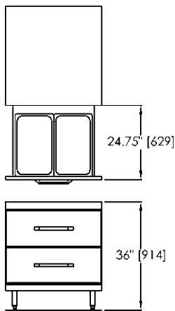
Model C11043-32E Increases standard 24" refrigerated section 8" to 32" - 29" or 33" deep bases. Supplied with (2) 12" x 20" x 6" dp. plastic pans per drawer.
