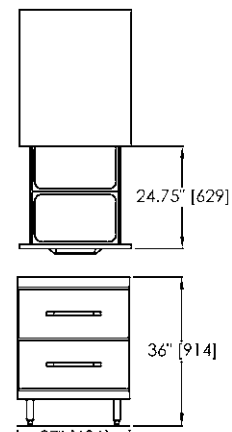
Model C11043-27E Increases standard 24" refrigerated section 3" to 27" - 33" deep bases only . Supplied with (2) 12" x 20" x 6" dp. plastic pans per drawer.
